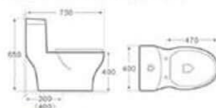
TR-1864 虹吸式單體馬桶 NT$24800 Size: 730X400X650mm 管距: 排污口中心離牆30,40cm
