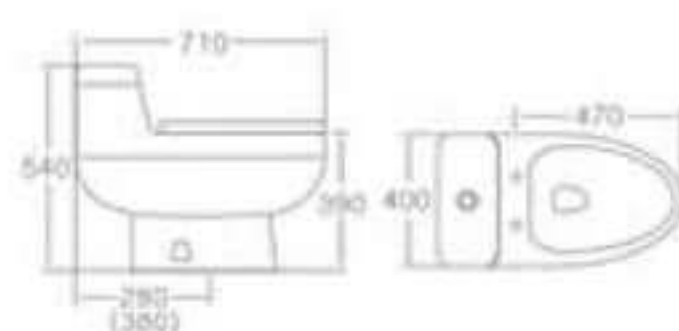
TR-632 虹吸式單體馬桶 NTS20400 Siphonic one-piece closet Size: 710x400x540mm S-trap, 30, 40cm Roughing-in
