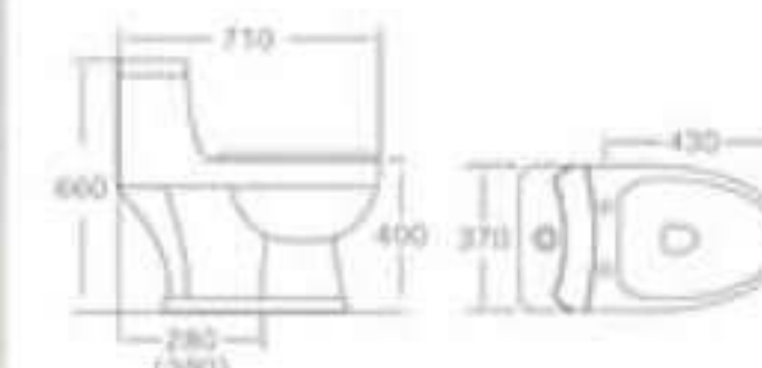
TR-2014 盥沖式單體馬桶 NTS18000 Washdown one-piece closet Size: 710x370x660mm S-trap, 30, 40cm Roughing-in
