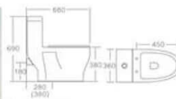
TR-645 盥沖式單體馬桶 NTS22000 Washdown one-piece closet Size: 680x360x690mm S-trap, 30, 40cm Roughing-in P-trap, 180mm Roughing-in
